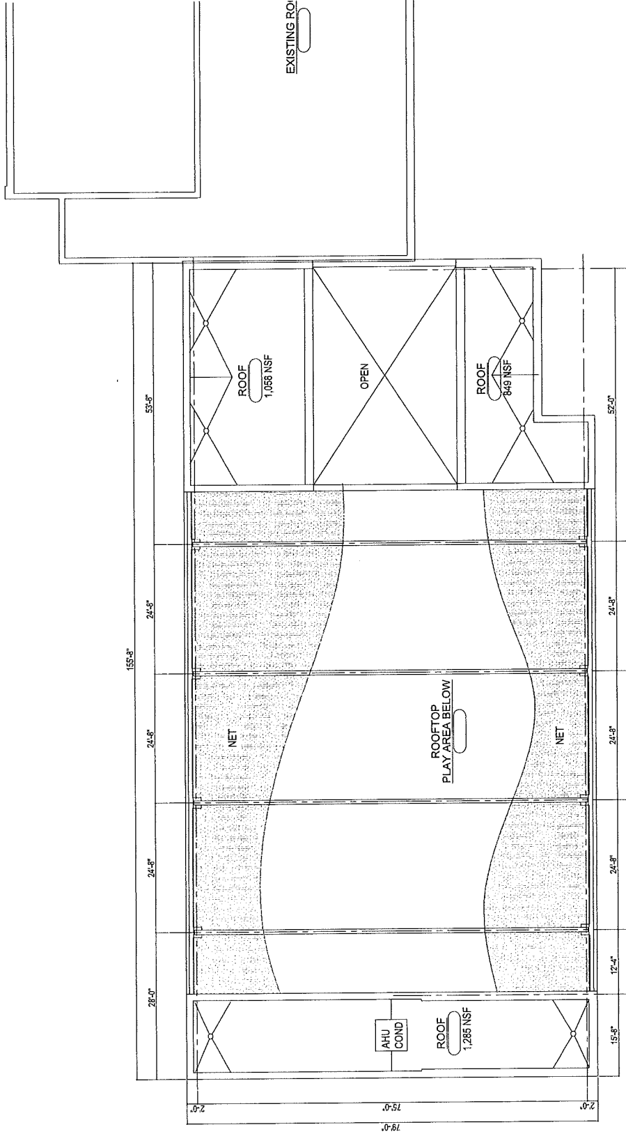
PROPOSED ANNEX ROOF PLAN GRAPHIC SCALE: 0 5 10 15 20 30 40 50 Lincoln ACR Agreement Miller-Huller
